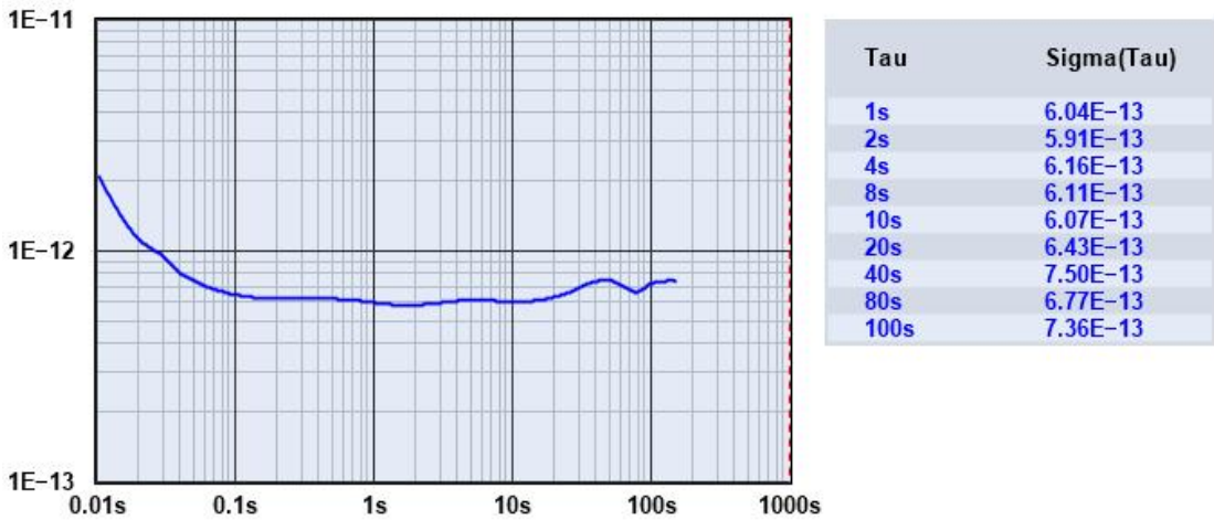
Allan Deviation \sigma_y(\tau)
